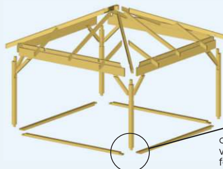
construction without ring beams
